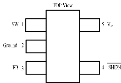
Fig. 2. IC LT 1615 as seen from the top [3].
