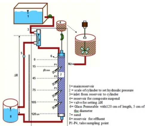
Fig 1. Packed Column Remediation
