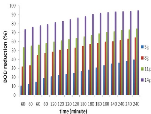
Fig.2. Effect of concentration of composite and contact time on BOD 5 reduction
