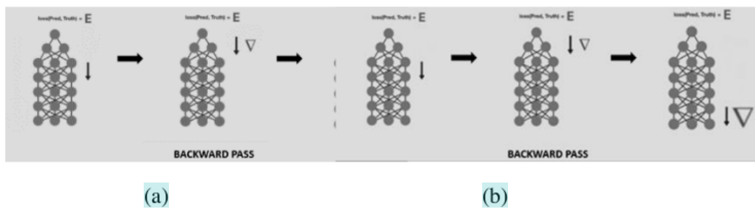
Gambar 4.13. (a) Vanishing Gradient , (b) Exploding Gradient
