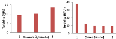
Figure 7. Testing turbidity levels (variation I)
