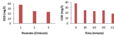
Figure 3. Testing of COD level (Variation I)
