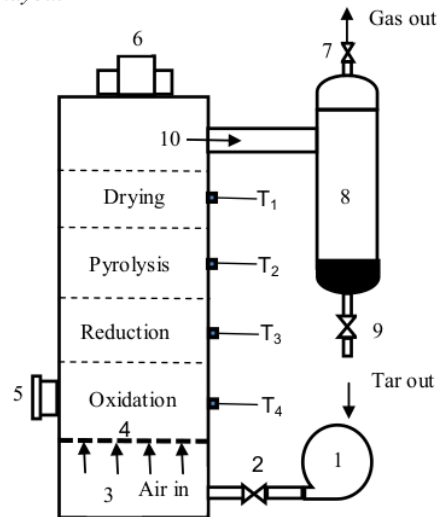
Figure 4. Experimental Equipment Schematic
