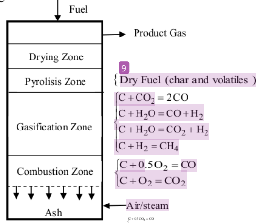
Figure 2. Updraft Gasifier Gasification Stages [2]
