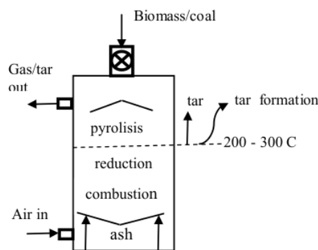
Figure 1. Updraft Gasifier
