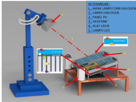
Gambar 1 Peralatan Penelitian.
