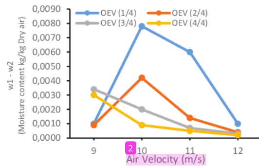
FIGURE 5. The effect of expansion valve opening and air velocity on moisture content
