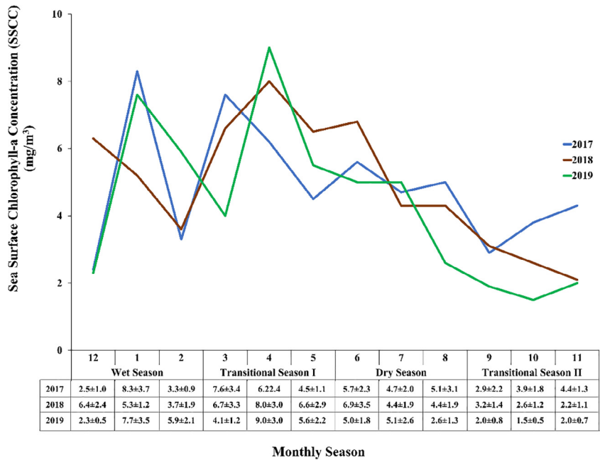
Fig. 5. Graph of fluctuation in the average distribution of sea surface chlorophyll-a concentration (SSC) in the waters of the Bangka Strait.
