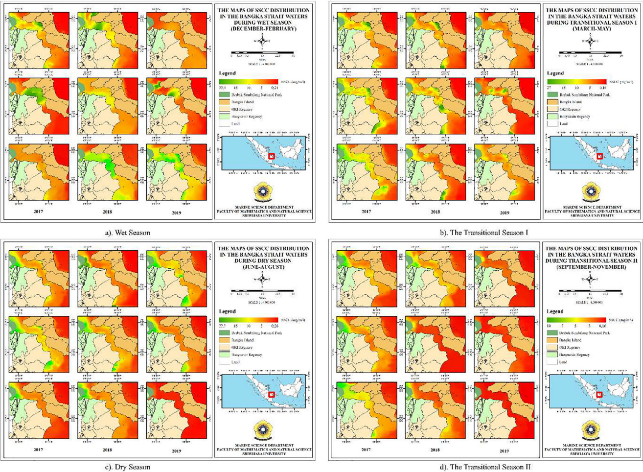
Fig. 4. The maps of SSC distribution: a) Wet Season (December-February); b) Transitional Season I (March-May); c) Dry Season (June-August); d) Transitional Season II (September-November).
