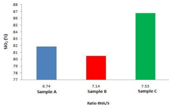
Figure 5: The effect of the ratio of RHA over the supporting material (S; bentonite and exfoliated graphite) in the RHG Samples
