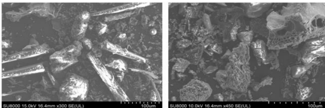
10 Fig. 1. SEM images of RH (a) and BC (b)
