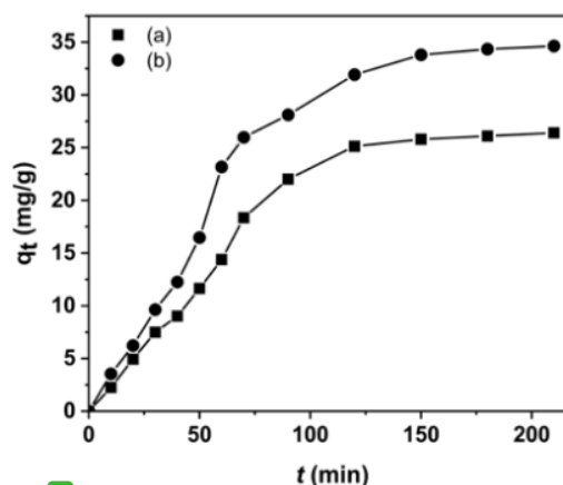
Fig. 6. Kinetic adsorption of Cr(VI) on RH (a) and BC (b); adsorbent dose = 0.25 g; volume adsorbate = 0.25 L; pH = 3.4 \pm 0.1 ; shaking speed = 180 rpm; initial concentration = 50 mg/L; temperature condition; 303 °K.
