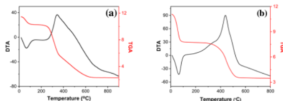
Fig. 4. TGDTA of RH (a) and BC (b)
