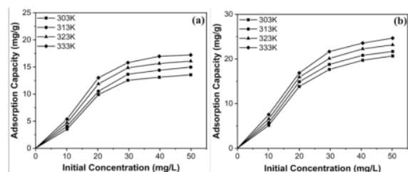
Fig. 5. Effect of initial concentration and temperature of Cr(VI) on RH and BC; adsorbent dose = 0.25 g; volume adsorbate = 0.25 L; shaking time = 120 min; pH = 3.4 \pm 0.1 ; shaking speed = 180 rpm;
