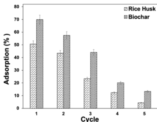
Fig. 7. Reusability of RH and BC on the adsorption of Cr(VI); adsorbent dose = 0.5 g; volume adsorbate = 0.25 L; shaking time = 30 min; pH = 2-4; shaking speed = 180 rpm; initial concentration = 50 mg/L; temperature condition; 303 °K.
