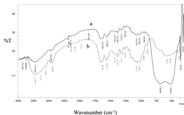
Figure 1. FT-IR Spectra for Chitosan-Ti/ZrO 2 (a) and Chitosan-ZrO 2 (b) Composite
