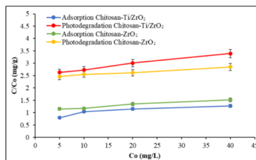
Figure 4. Graph of Comparison Between Removal Efficiency of Pesticide Paraquat Dichloride by Composite Materials using Adsorption and Photodegradation Treatment
