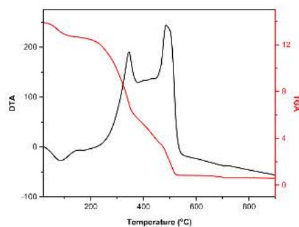
Figure 5. TG-DTA Profile of Longan ( Dimocarpus longan )
