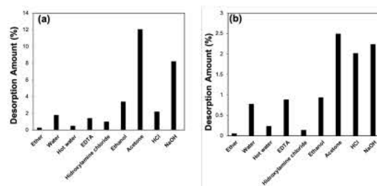
Figure 12. Desorption Process of Malachite Green (a) and rhodamine-B (b)
