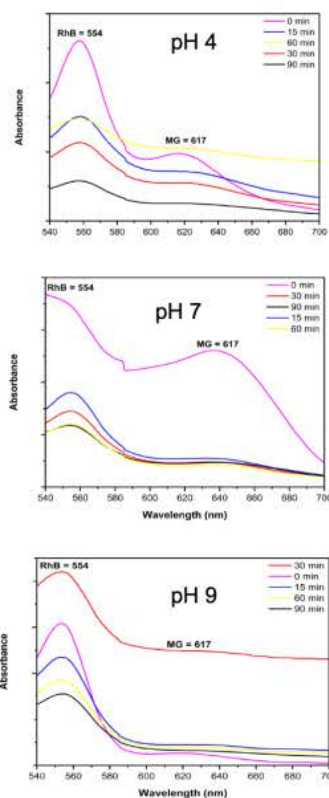
Figure 8. UV-Vis Spectrum of Dyes Mixtures After Adsorption at Several Times
