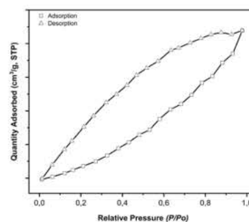
Figure 4. N 2 Isotherm Adsorption-Desorption of Logan ( Dimocarpus longan )
