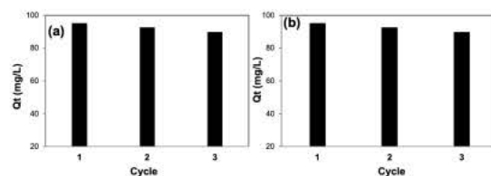
Figure 13. Cycling Bioadsorbent After Adsorption of Malachite Green (a) and Rhodamine-B (b)
