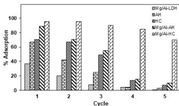
Figure 7. Regeneration of Mg/Al LDH, AH, HC, Mg/Al-AH, and Mg/Al-HC
