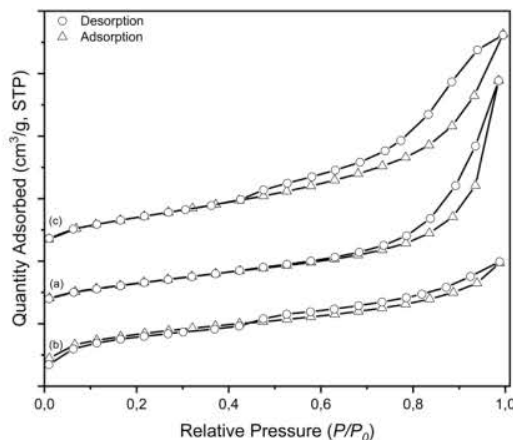
FIGURE 2. \text{N}_2 adsorption-desorption curve of (a) CuAl LDH, (b) BC, (c) CuAl-LDH@BC composite
