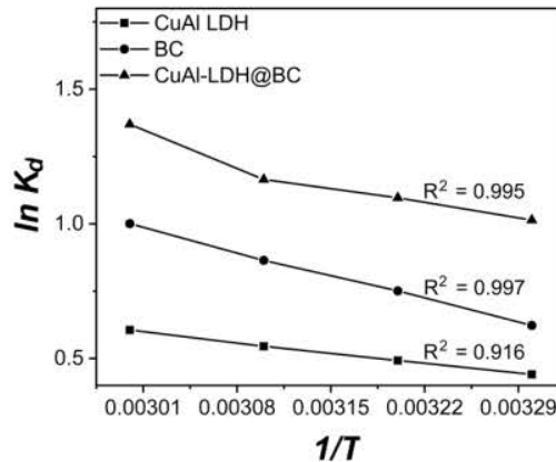
FIGURE 7. Van't Hoff Plot of CR adsorption onto CuAl LDH, BC and CuAl-LDH@BC
