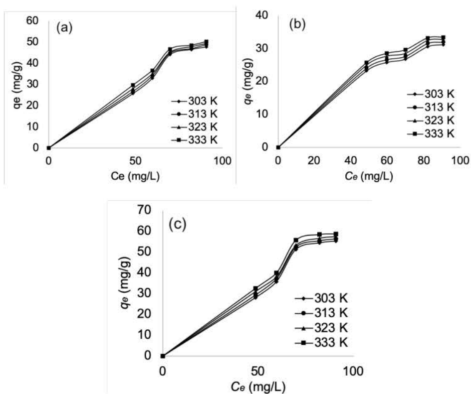
FIGURE 6. Effect of initial temperature of CR adsorption onto CuAl LDH (a), BC (b), CuAl LDH@BC composite (c)
