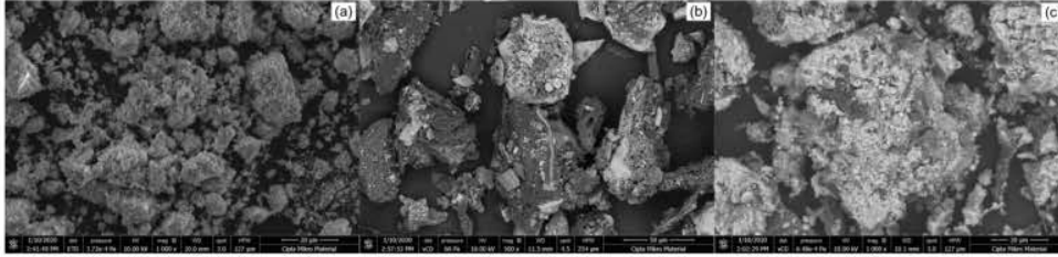
FIGURE 4. SEM images of (a) CuAl LDH, (b) BC, (c) CuAl-LDH@BC composite
