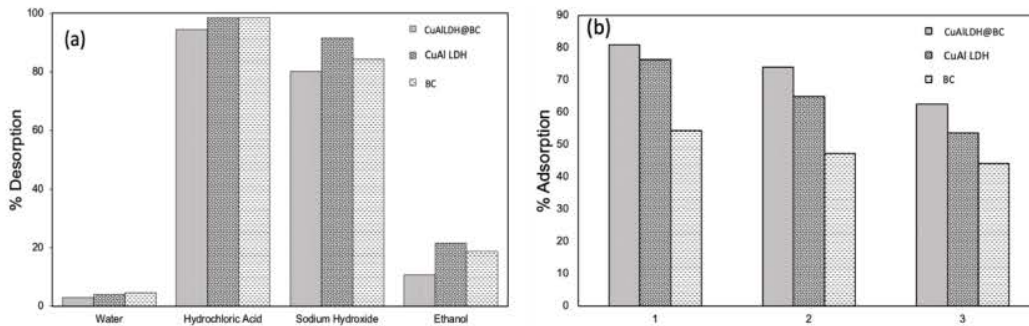
FIGURE 8. (a) CR desorption study and (b) regeneration of adsorbents
