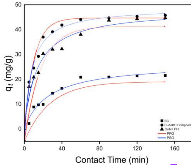
FIGURE 5. The curve of fitted kinetics model against the experimental data by CuAl LDH, BC, and CuAl-LDH@BC composite
