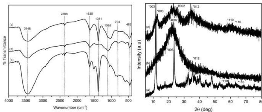
FIGURE 1. FTIR spectra and XRD pattern of (a) CuAl LDH, (b) BC, (c) CuAl-LDH@BC composite
