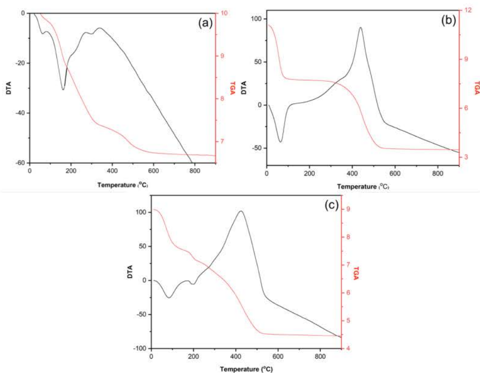
FIGURE 3. Thermogravimetry curve of (a) CuAl LDH, (b) BC, (c) CuAl-LDH@BC composite
