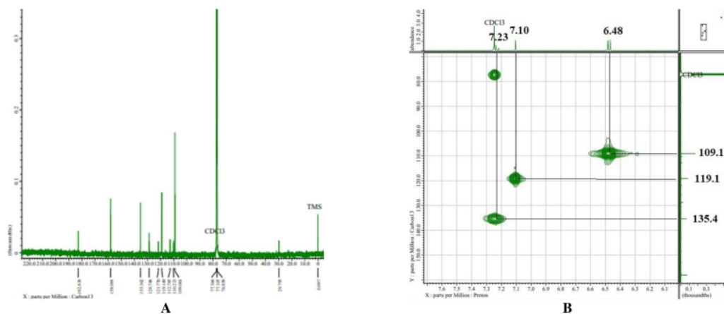
Figure 4. The ^{13}\text{C-NMR} (A) and HMQC (B) spectrum of compound 1 ( ^1\text{H} -500 MHz; ^{13}\text{C} -125 MHz in \text{CDCl}_3 )
