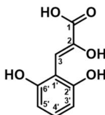
Figure 4. The structure of compound 1 as 3-(2,6-dihydroxyphenyl)-2-hydroxyacrylic acid
