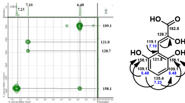
Figure 5. The HMBC spectrum of compound 1
