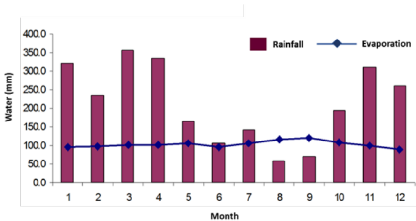
Figure 3. Relationship Between Rainfall and Monthly Potential Evapotranspiration
