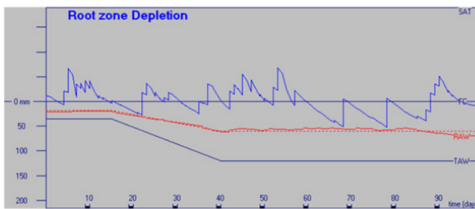
Figure 10. Irrigation simulation during March - June 2015
