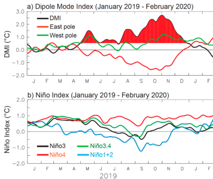
Figure 1. Time series of (a) Dipole Mode Index (black), eastern (red), and western (green) poles indices; and (b) Niño indices from January 2019–February 2020. Note that the red shading area indicates the DMI value above one standard deviation.
