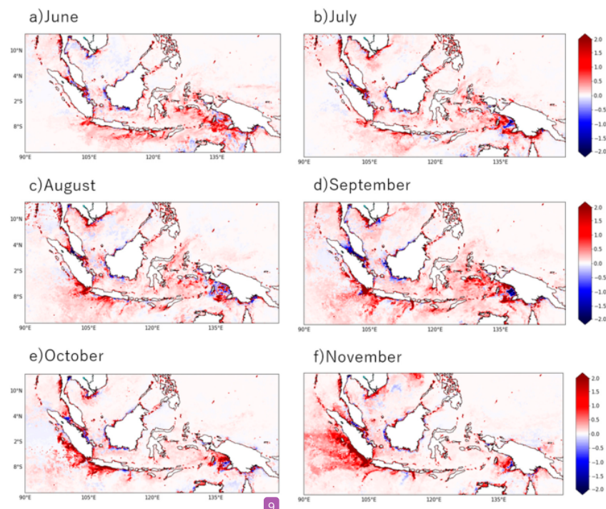
Figure 9. Monthly anomaly of the surface chlorophyll-a concentration ( \text{mg m}^{-3} ) within the Indonesian seas during June–November 2019.
