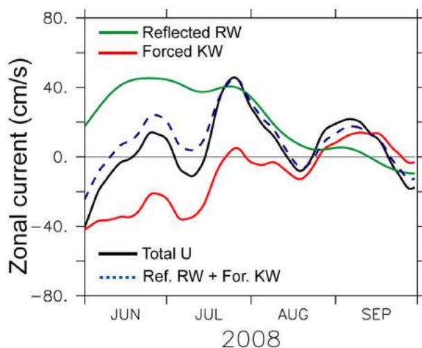
Fig. 8. Time series of zonal current anomaly at 15-m depth averaged over the region of ( 80^{\circ}\text{E} - 93^{\circ}\text{E} , 4^{\circ}\text{S} - 2^{\circ}\text{N} ) for June-September 2008 from reflected Rossby wave (green), forced Kelvin wave (red), total solution (black), and the sum of reflected Rossby and forced Kelvin waves (blue-dashed)
