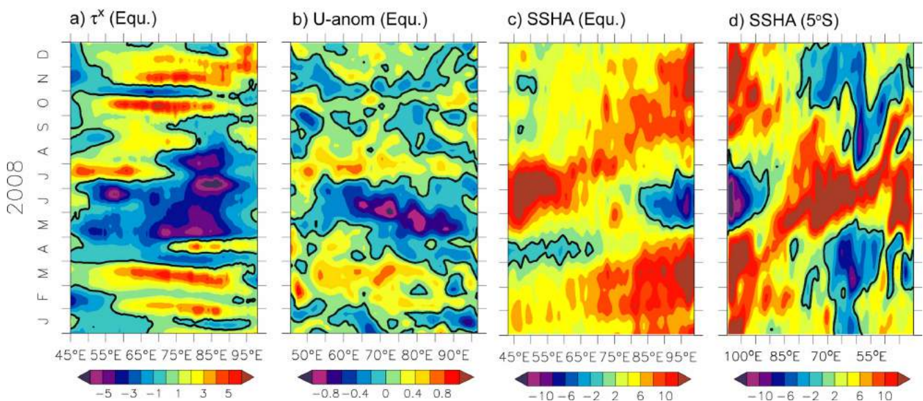
Fig. 6. Time-longitude diagrams of (a) zonal wind stress anomaly ( \times 10^{-2} N/m 2 ), (b) zonal current anomaly (m/s), (c) SSH anomaly along the equator (cm), and (d) SSH anomaly along 5°S (cm). The zero contour is highlighted by thick-black contour. The anomalies are obtained by subtracting the mean climatologies, then smoothing with a 15-day running mean filter
