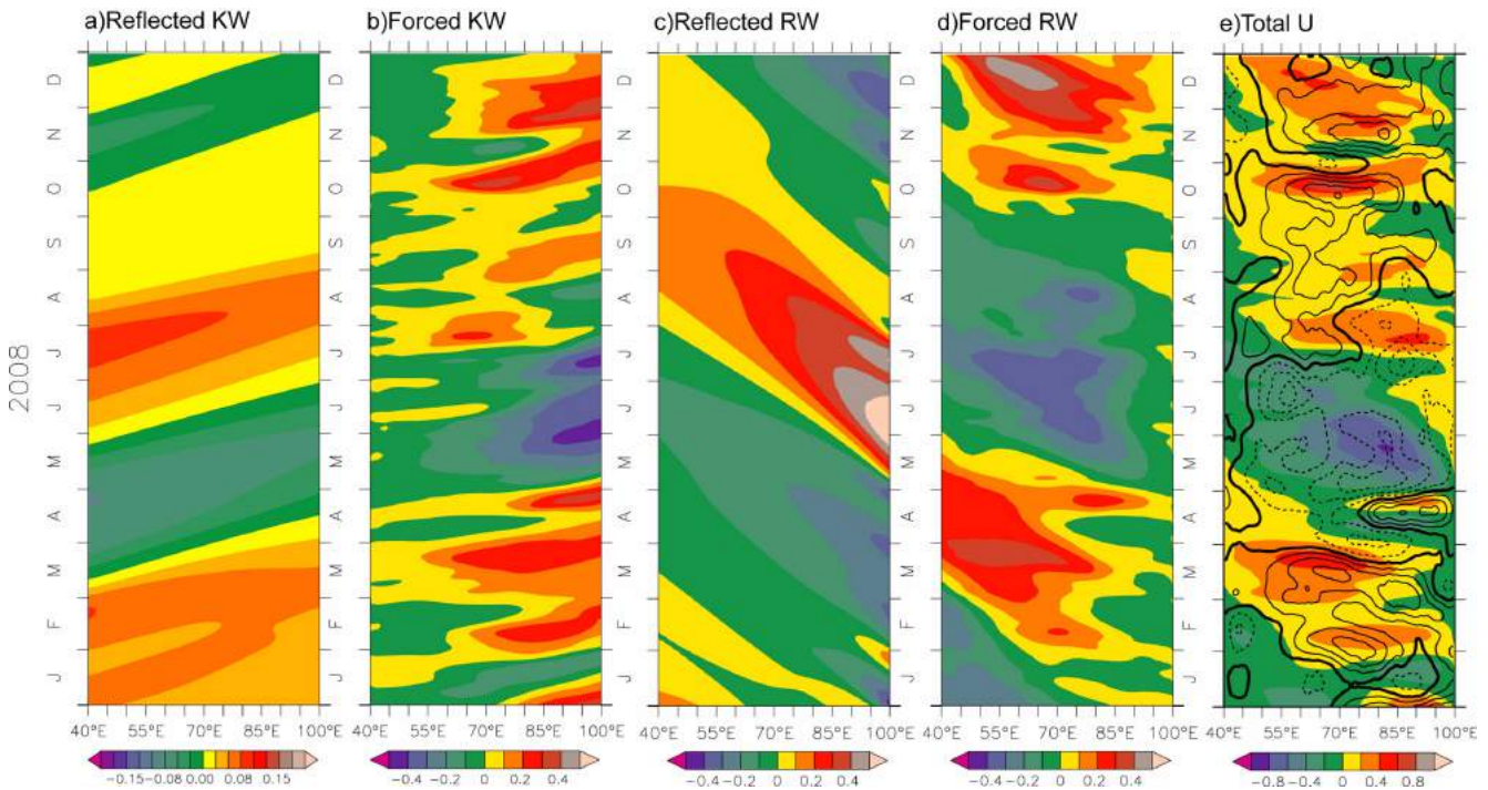
Fig. 7. Time-longitude diagrams of model zonal current anomalies at 15 m depth along the equator for January-December 2008, from (a) reflected Kelvin waves, (b) wind-forced Kelvin waves, (c) reflected Rossby waves, (d) wind-forced Rossby waves, and (e) total. The contours in Figure 8e show anomalies of zonal wind stress along the equator. The solid (dotted) lines are for westerly (easterly) anomalies. Contour interval is 1.5 \times 10^{-2} \text{ N/m}^2 with zero contour highlighted. Note the scales change in (a) and (e)
