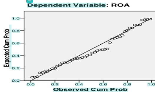
Gambar 4.1 Grafik normal P-P Plot of Regression Statistics
