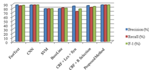
Figure 4. Result of comparison with Bustos [21] and Moharasan [34]
