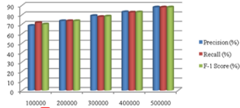
Figure 3. Graph of CRF with bigram
