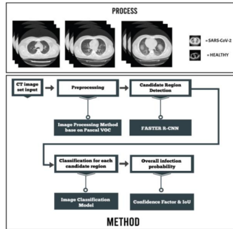
Fig. 4. The process of infected lesion detection.
