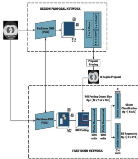
Fig. 5. The Faster-RCNNs architecture.
