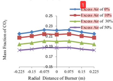
Fig. 9. Carbon dioxide distribution on middle of gas burner at radial distance with difference excess air.
