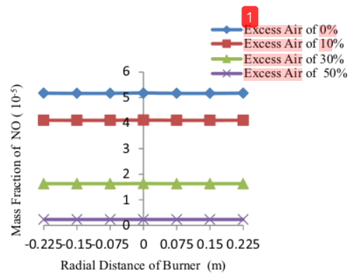
Fig. 19. Nitric Oxide distribution on middle of gas burner at radial distance with difference excess air.
