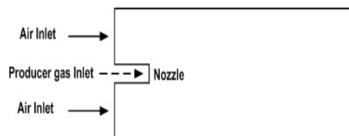
Fig.1. The scheme of gas burner
