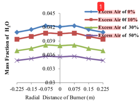
Fig. 14. Water vapor distribution on middle of gas burner at radial distance with difference excess air.
