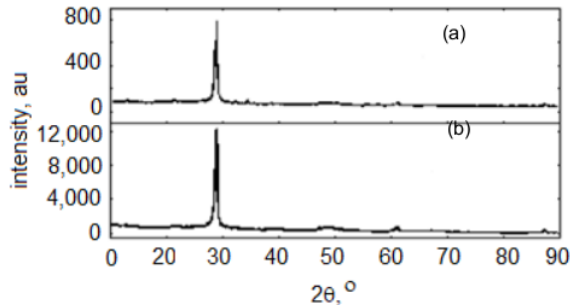
Figure 2: The diffractogram of the electrode with carbon nanosheet – graphite ratio of (a) 3:7 and (b) 7:3
