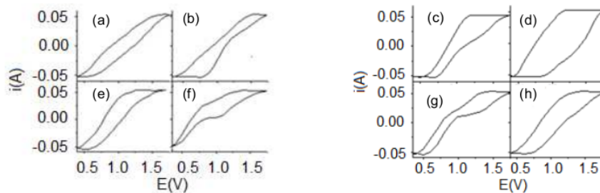
Figure 3: Voltammograms of the electrodes with carbon nanosheet:graphite ratio of 3:7 at various concentration of electrolytes measured at scan rate 20 \text{ mV s}^{-1} : (a) 10 % lithium chloride (b) 20 % lithium chloride (e) 10 % ammonium cyanate (f) 20 % ammonium cyanate; with carbon nanosheet:graphite ratio of 7:3 at various concentration of electrolytes measured at scan rate 20 \text{ mV s}^{-1} : (c) 10 % lithium chloride (d) 20 % lithium chloride (g) 10 % ammonium cyanate (h) 20 % ammonium cyanate
