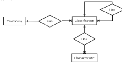
Figure 3. Entity Relationship Diagram
