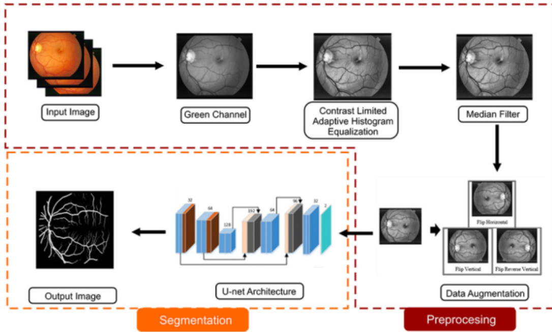
21 Fig. 1. Flowchart of the proposed method for data augmentation on vascular retinal image segmentation.
