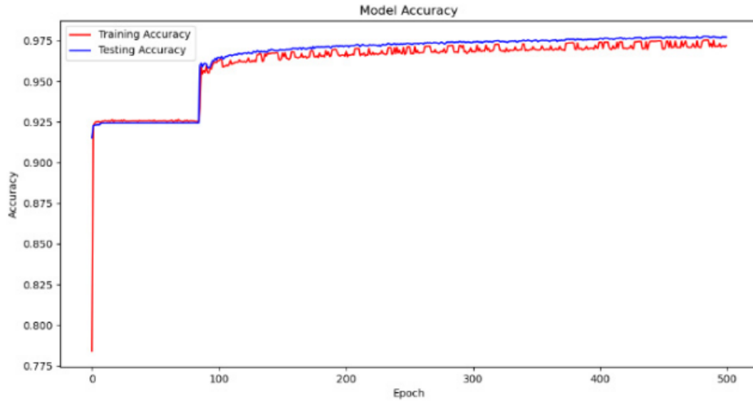
Fig. 7. Graph of training and testing process accuracy.
