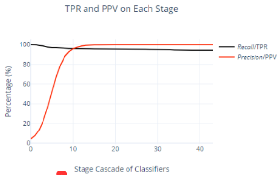
1 Stage Cascade of Classifiers Fig. 10. Recall and precision charts.
