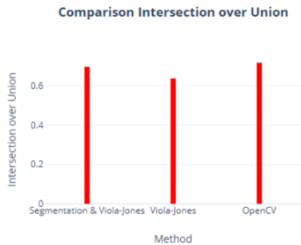
Fig. 11. Comparison of Intersection over Union (IoU).
