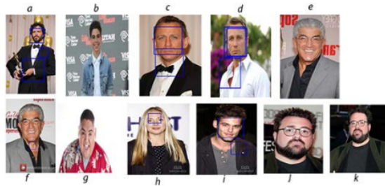
Fig. 12. Viola-Jones results.
