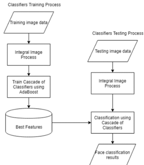
Fig. 5. Stages of training process.
