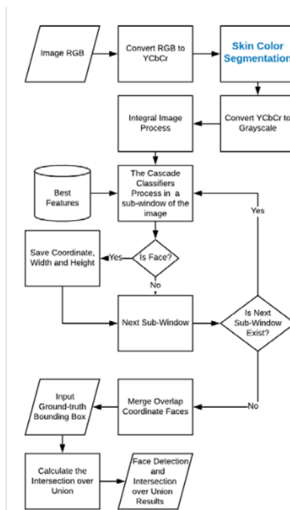
Fig. 6. Face detection process.
