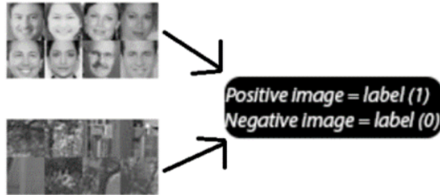
Fig. 7. Data training.
