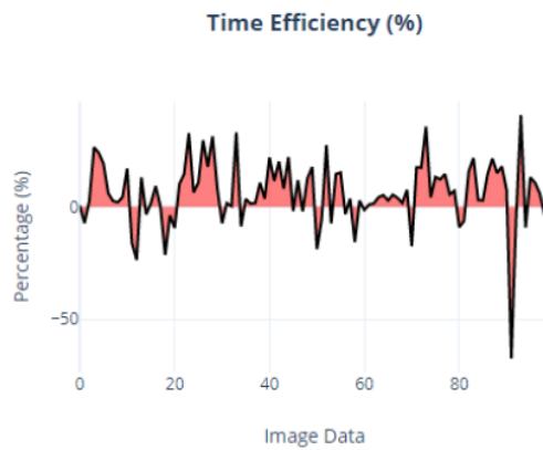
Fig. 15. Time efficiency.
