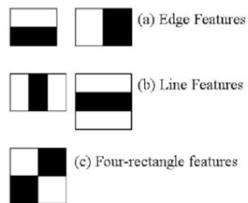
Fig. 2. Haar-like features.
