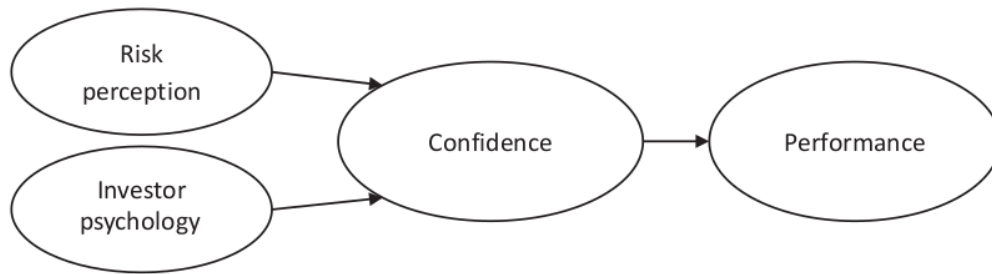
Figure 1. Research model
