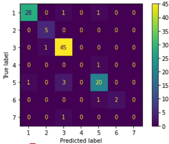
Fig. 10. Confusion Matrix of Data Testing Results.
