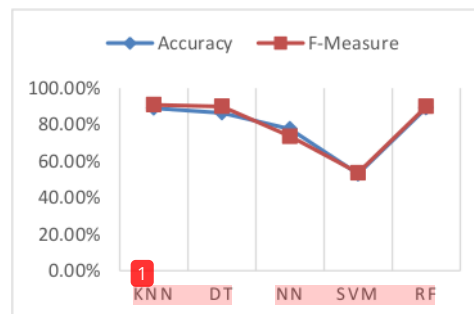
Fig. 9. Machine Learning Models Performance Comparison Visualization.
