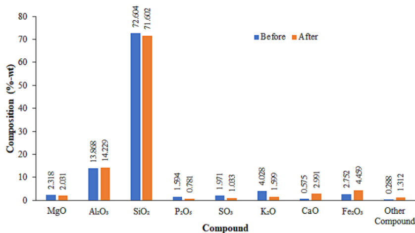
Figure 3. Chemical composition of bottom ash before and after adsorption
