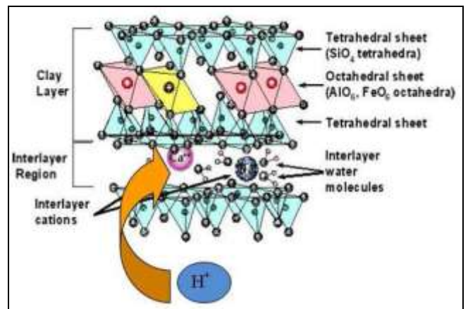
Fig 1: Bentonite reaction of HCl activation
