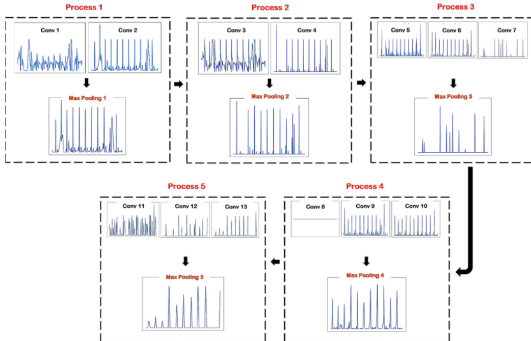
Fig. 6. Features map from convolution and max-pooling process.
