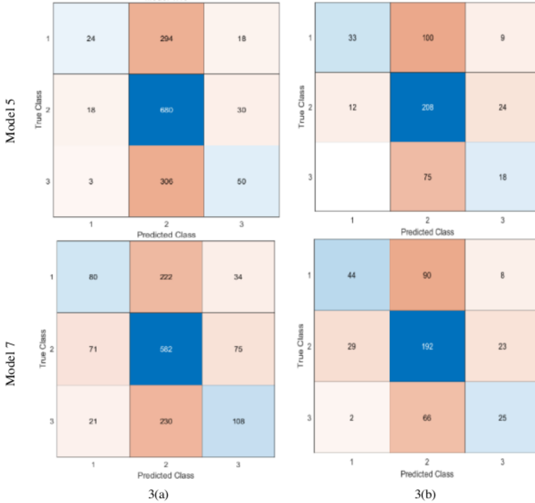
Fig. 3. Confusion matrix of the (a) training data (b) test data
