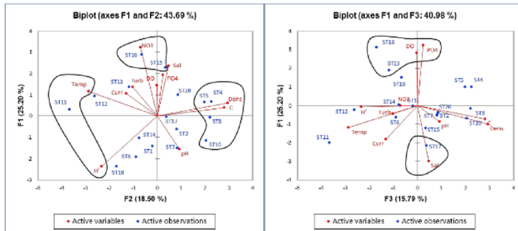
Figure 6. Principal Component Analysis
