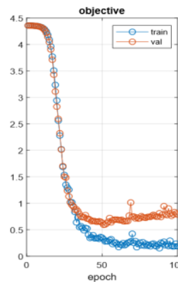
Figure 5. Training Graphs of the Objective Function for 100 Epochs Without Dropout (above) and With Dropout (below)
