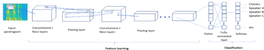
Figure 3. Architecture of the Convolutional Neural Network (CNN)
