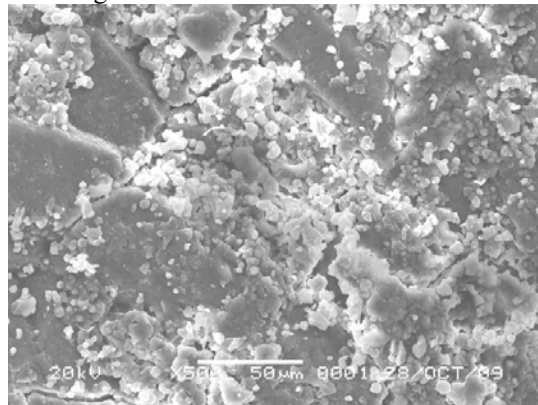
Figure 5. Scanning electron micrograph of IR 42 variety (x 500).
