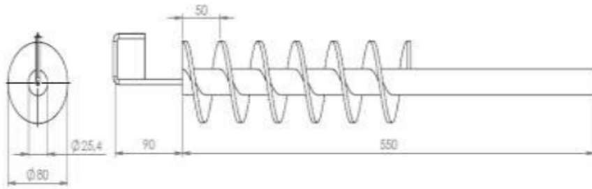
Screw
