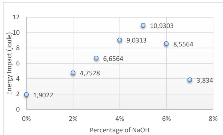
Figure 8. Result of impact test
