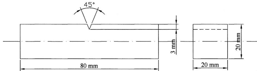
Figure 7. Impact standar ASTM E 23-88
