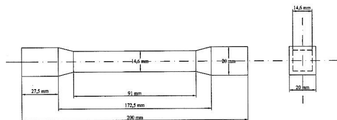
Figure 4. Specimen standar of ASTM 638-90
