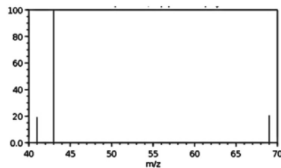
1-(Methylcyclopropyl)-ethanol Anticancer
