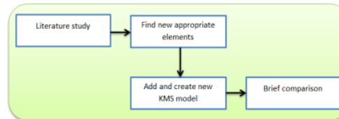
Fig. 4: Research steps
