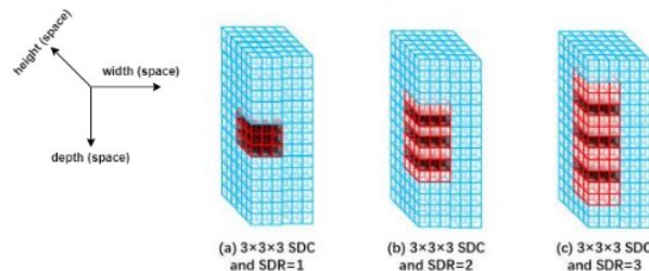
Gambar 7. Dilated Convolution 3 Dimensi [16]
