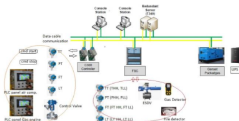
Figure 3 Architecture DCS ( input and output)
