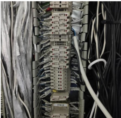
Figure 8 Terminal cable connected field JB to Digital Output (Relocated the most crowded load terminal to single load terminal)
