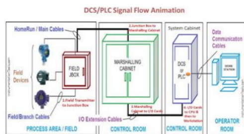
Figure 1 DCS/PLC Sinyal Flow Animation
