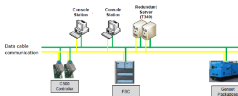
Figure 2 Architecture DCS at PT Pertamina EP Asset 2
