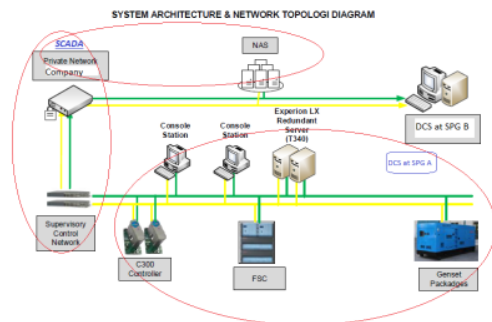
Figure 4 System Architecture & Network Topology Diagram
