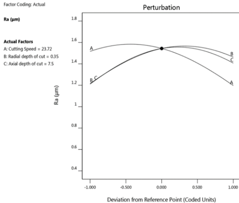
FIGURE 3. The perturbation plot for surface roughness
