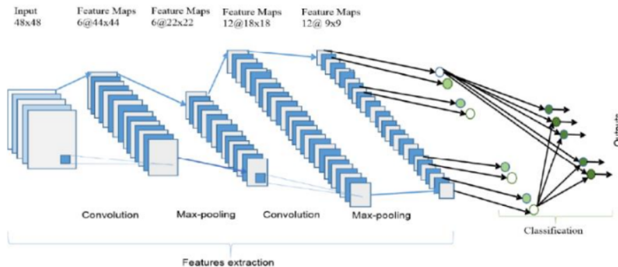
FIGURE 2. CNN Process
