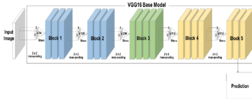
FIGURE 3. VGG-16 Architecture [27]
