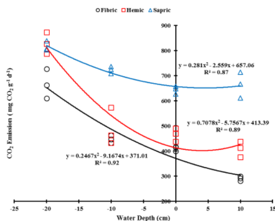
Figure 1. Effect of water levels on \text{CO}_2 emissions from peat soil with different levels of humification (Values are based on n = 15 ).
