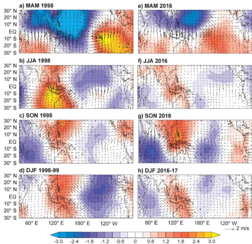
Fig. 3 Same as Fig. 2, but for velocity potential anomalies ( shaded ; 10^5 \text{ m}^2 \text{ s}^{-1} ) and convergent/divergent winds anomalies ( vector ; \text{m/s} ) at 850 mb.
