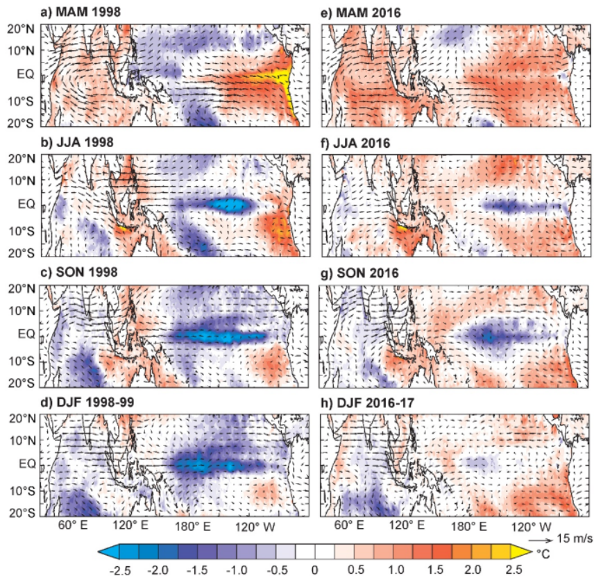
Fig. 2 Seasonally averaged of SST anomalies ( shaded ; °C) and winds anomalies ( vector ; m/s) during 1998-99 (left) and 2016-17 (right) in (a,e) boreal spring (MAM), (b,f) boreal summer (JJA), (c,g) boreal autumn (SON), and (d,h) boreal winter (DJF), respectively.
