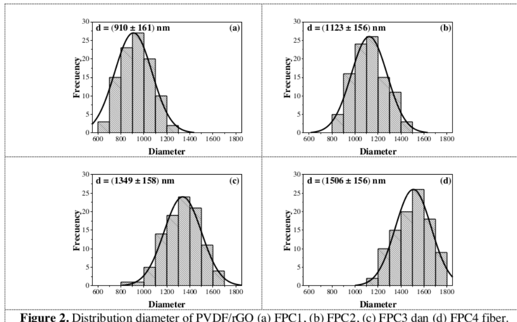
Figure 2. Distribution diameter of PVDF/rGO (a) FPC1, (b) FPC2, (c) FPC3 dan (d) FPC4 fiber.
