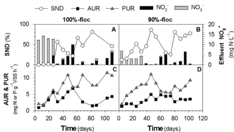
Fig. 5. SBR performance comparison of SND efficiencies, effluent nitrate and nitrite levels, ammonium uptake rates (AUR) and phosphorus uptake rates (PUR) from the 100%-floc (A and C) and the 90%-floc (B and D) SBRs.
