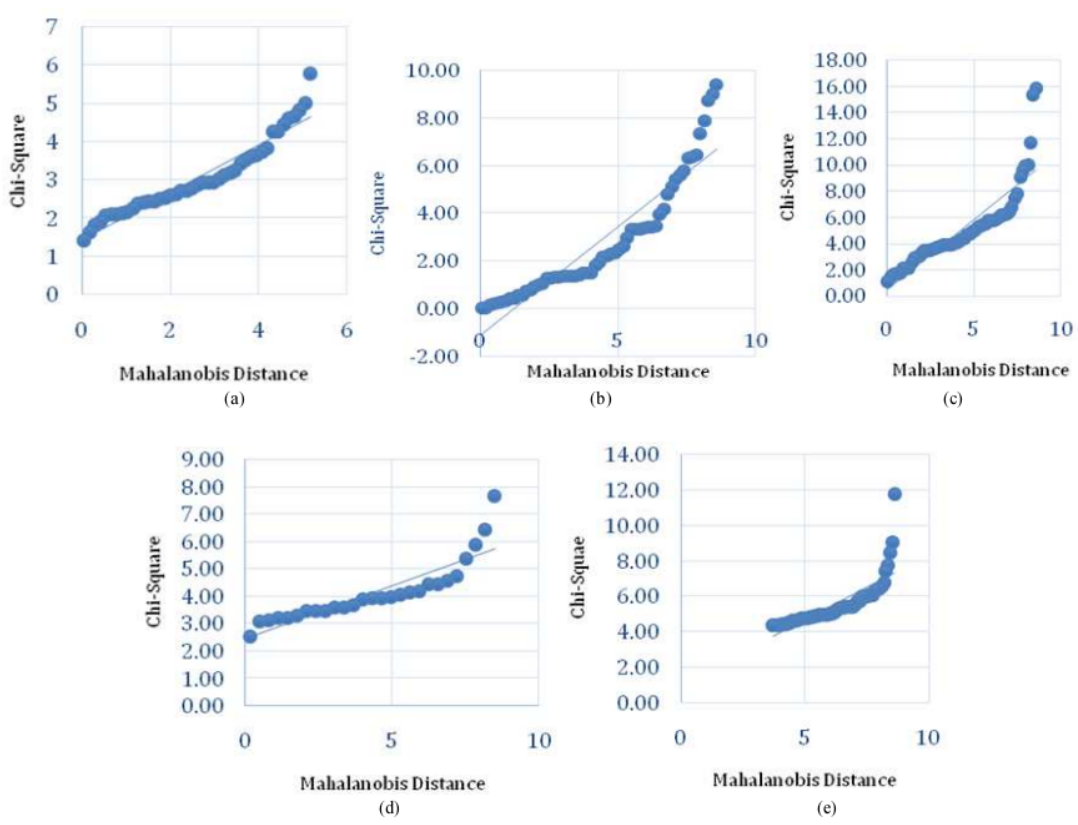
Fig. 1. Plot Mahalanobis Distance for (a) South, (b) Center, (c) North, (d) West, (e) East
