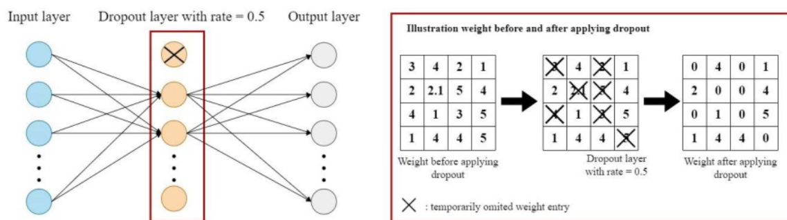
FIGURE 8. Example of a simple calculation on the dropout layer on the proposed architecture VG-DropNet.
