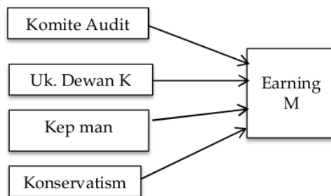
Gambar 1. Rerangka Penelitian
